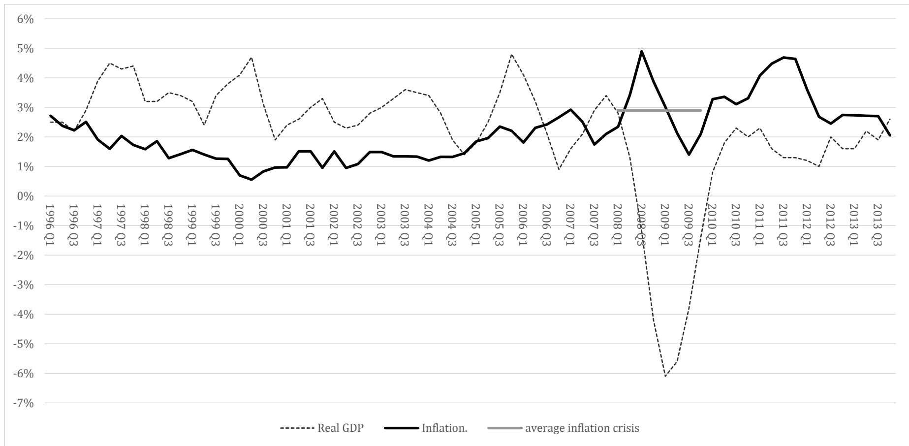
Figure 1: Quarterly inflation and output growth 1996-2013.
