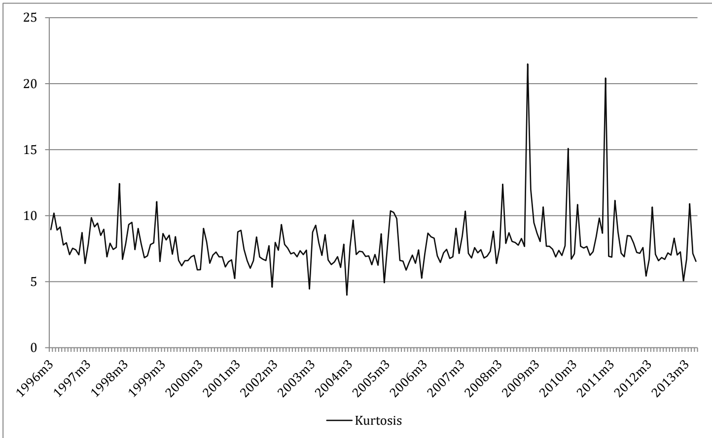
Figure 5: The time series of kurtosis
