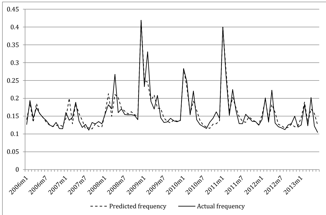
Figure 6: Actual and predicted frequency of price changes 2006-2013
