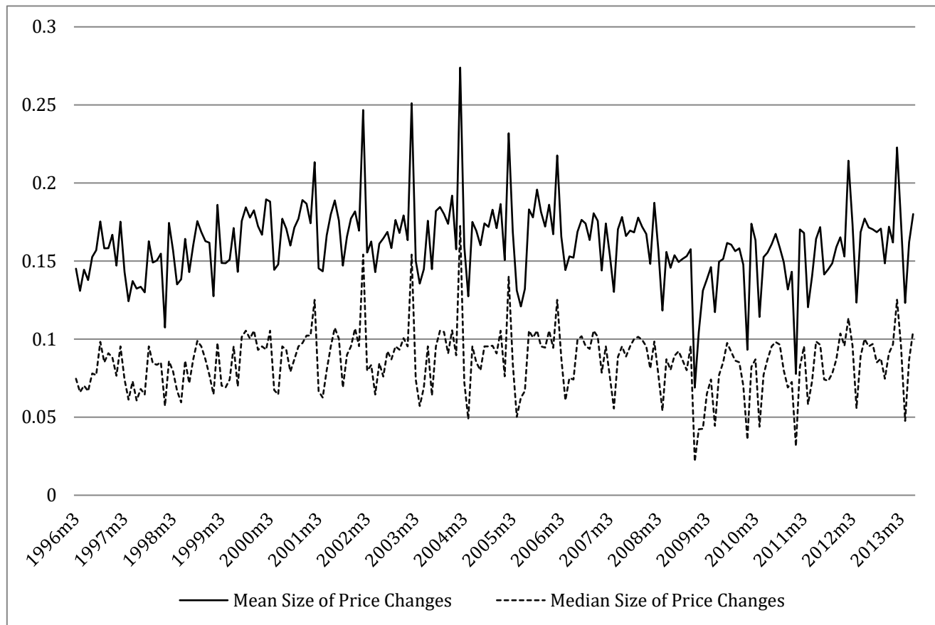
Figure 4A: The time series of absolute price growth
