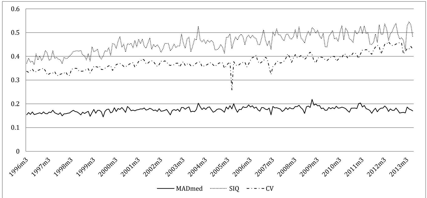
Figure 3: The time series of price-level dispersion measures MADmed, SIQ, and CV.
