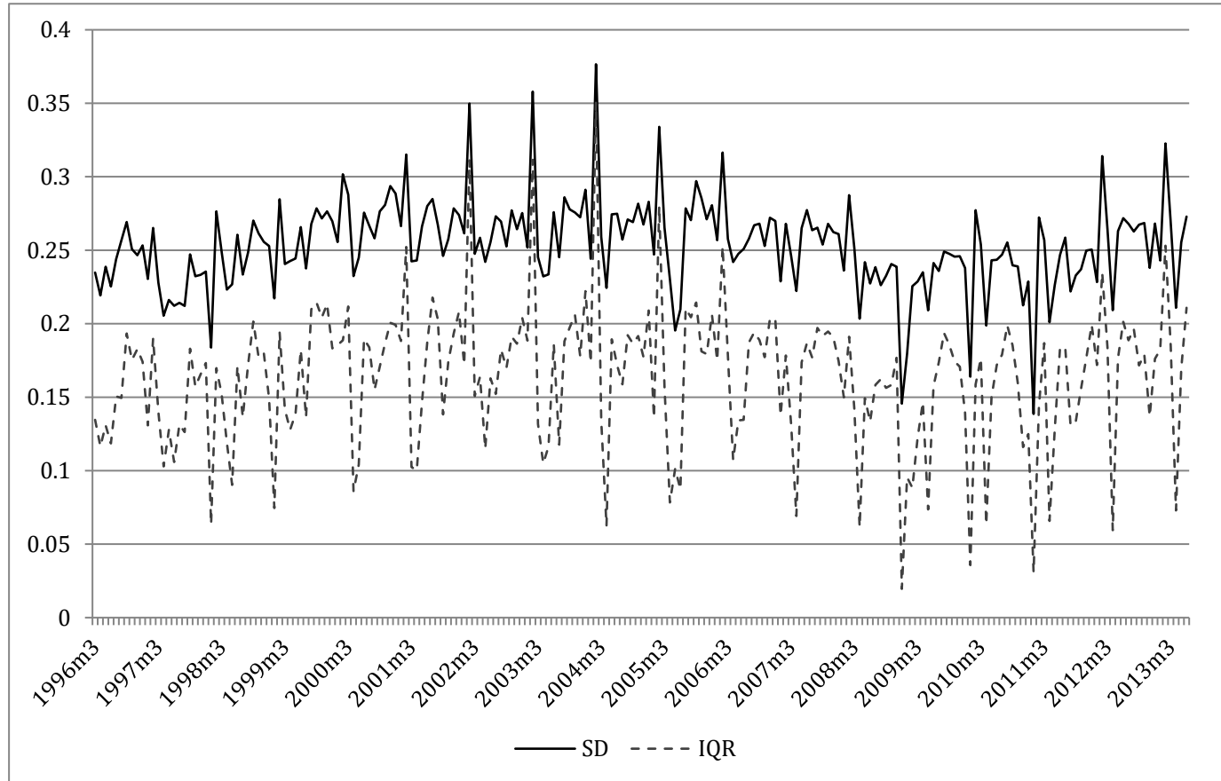
Figure 4B: The time series of price-growth dispersion Note: “SD” denotes standard deviation, and “IQR” the interquartile range.
